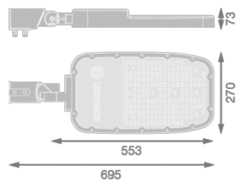
SL AREA SPD 150W
