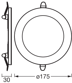
DL SLIM175 RD ADJ SIDE-MAIN 830 WT
