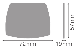
TRUSYS FLEX END CAP LOW
