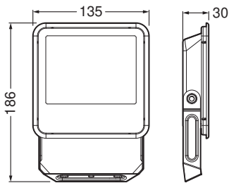
LED ECO LITE FLOODLIGHT 30W
