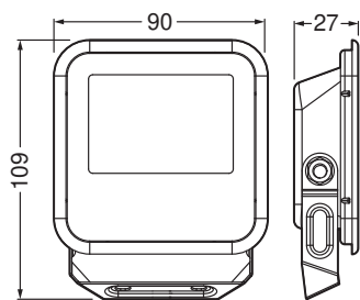
LED ECO LITE FLOODLIGHT 10W
