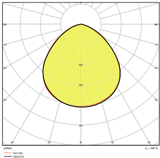
LDVAL FL 30 W 6500 K GEN2
