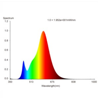
EPREL data spectral diagram PROF LEDr 2700K
