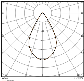
HB DA P 75W 840 70DEG IP66 WITH REFRACTOR
