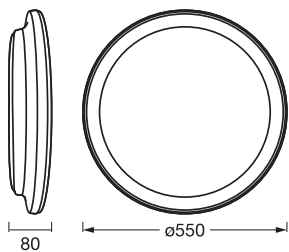
ORBIS PEDERSON 550MM 36W 830
