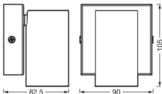
LED SPOT OCTAGON 1X3.4W 927 GU10
