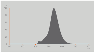
EPREL Data Spectral Diagram LEDr _1800K_1906_Vintage_Smoke
