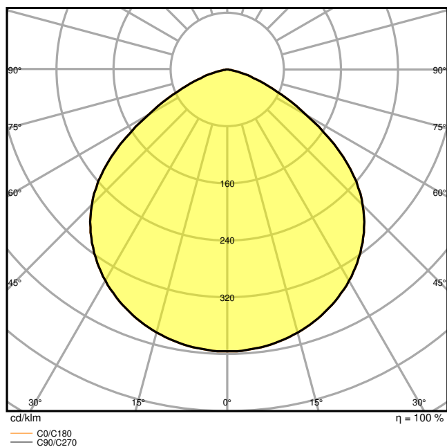
HB-DALI-93W-4000K-110DEG-IP65
