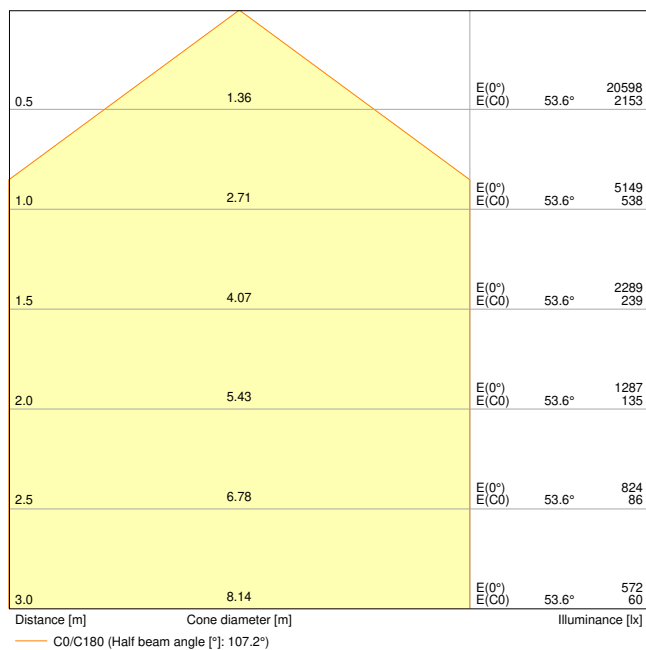
HB-DALI-93W-4000K-110DEG-IP65
