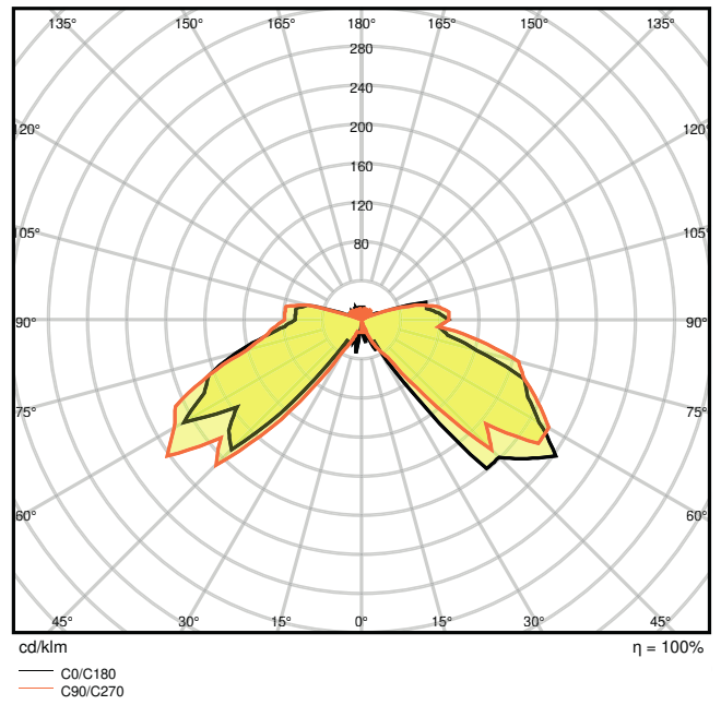
4058075075177 O Surface Pole 6W3000K SST IP44
