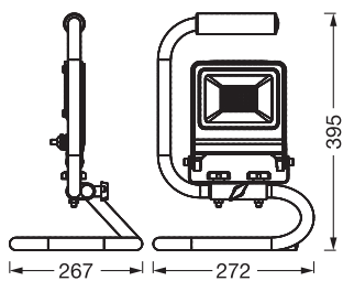
LED WORKLIGHT 50W S-STAND CH PLUG OSRAM
