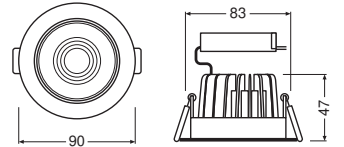
707987_LEDVANCE Spot LED adjust 8W
