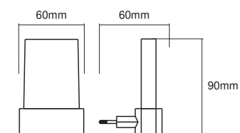
Produkt Line Drawing LUNETTA Shine WT
