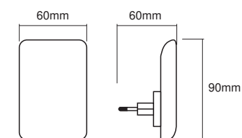
Produkt Line Drawing LUNETTA Glow White
