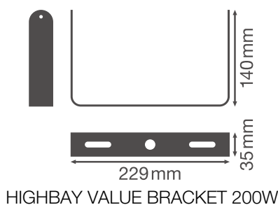
HIGHBAY VALUE BRACKET 200W
