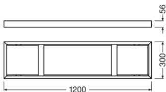
PANEL 1200 SURFACE MOUNT KIT
