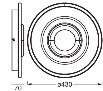
ORBIS CRISTALLY 430MM 50W CCT WT
