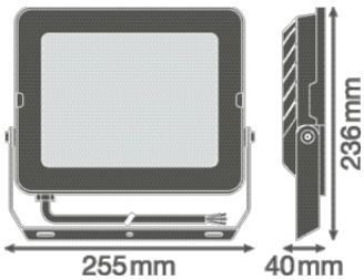
FL COMP V 90W 830 SYM 100 BK
