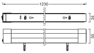
LED BATTEN 120CM 16W 840 G13 T8
