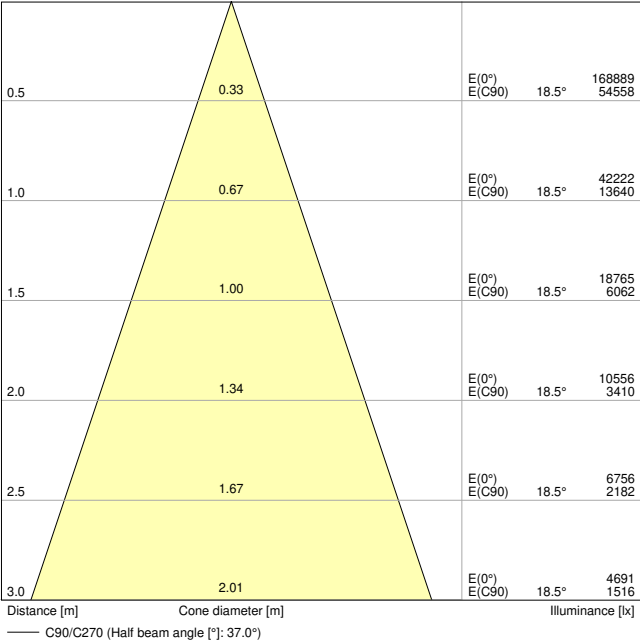
LEDVANCE FLOODLIGHT SYM 160W 36D
