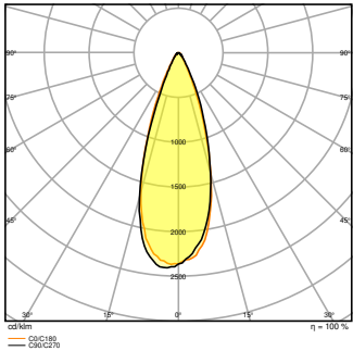
LEDVANCE SPOTLIGHT 10W 840 36D G2
