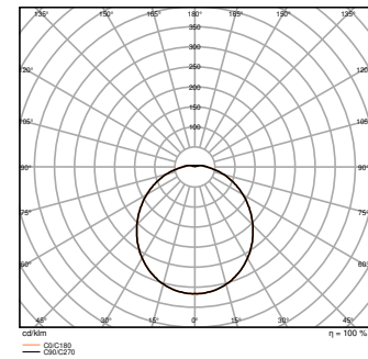
DP CBO 1800 V 60W MS 840 IP66 GY
