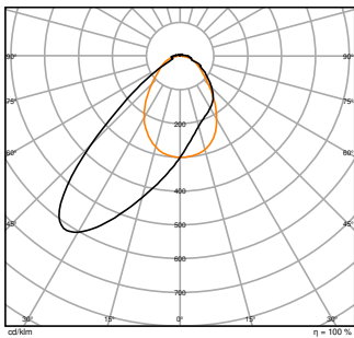
TRUSYS FLEX P 50W 865 WW CL WT
