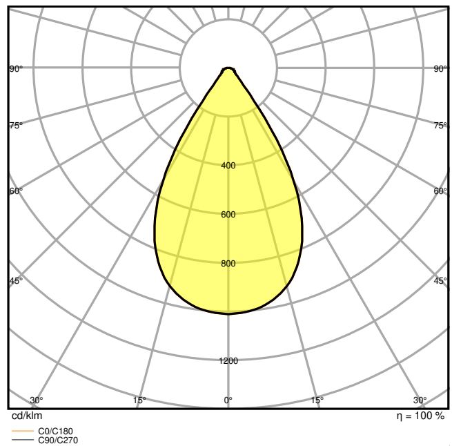
HB-DALI-190W-4000K-70DEG-IP65
