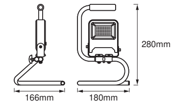
LED WORKLIGHT 20W S-STAND
