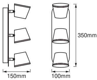
LED SPOT 3X7W IP44 30CM
