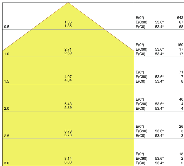
Distance [m] Cone diameter [m] Illuminance [lx] — C0/C180 (Half beam angle [°]: 106.8°) — C90/C270 (Half beam angle [°]: 107.2°)
