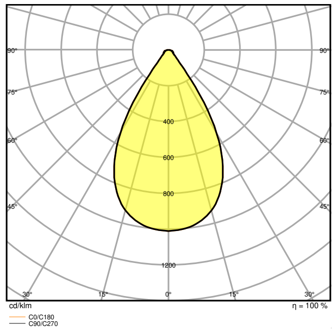
HB-DALI-190W-4000K-70DEG-IP65
