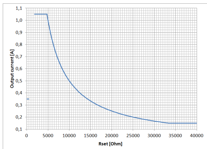
Typical Iout vs Rset
