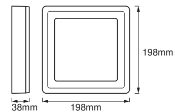
LED CLICK WHITE SQ 200MM 16W
