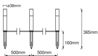
SMART WIFI GARDEN POLE RGBW 3PEXT
