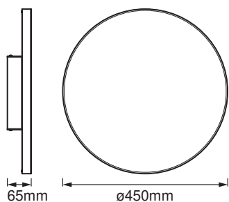
SMART WIFI PLANON FRAMELESS RD45 TW
